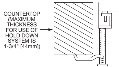
Cross Profile of Installation
